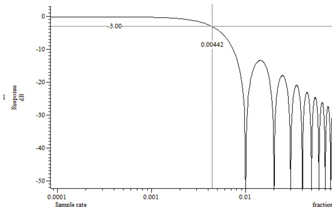
Frequency response of smoothing filter (n=100). Frequency expressed as a fraction of the sampling rate.
